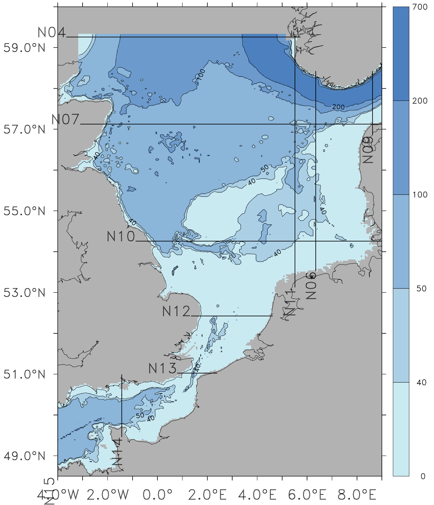
N00S sections, North Sea
